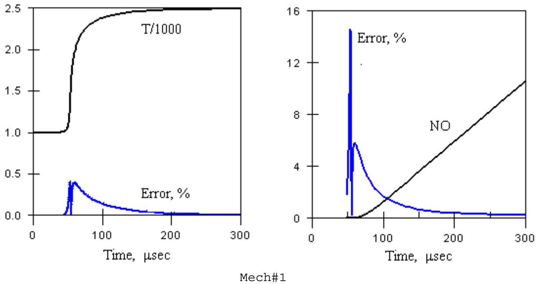
Fig. 2.1 Temperature, T(K)/1000 and relative error, % Fig. 2.2. NO concentration, mol/cm 3 × 1.E+11 and relative error, %
