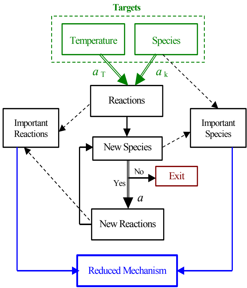
Fig. 1.1. Selection of important species and reactions on a single time interval
