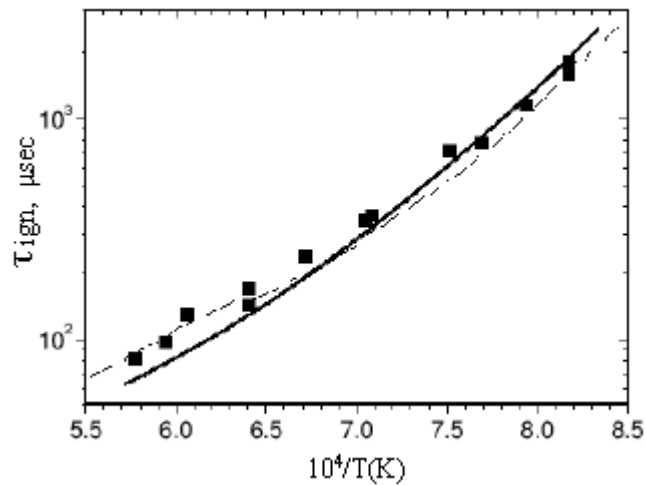
Fig. 2.9. Ignition delay time; experimental (symbols) and computed (solid line) data from [9], dotted line – this calculation. \text{C}_2\text{H}_4 – 0.5%, \text{O}_2 – 1.5 %, Ar – 98%, P_5 = 1.07 atm.
