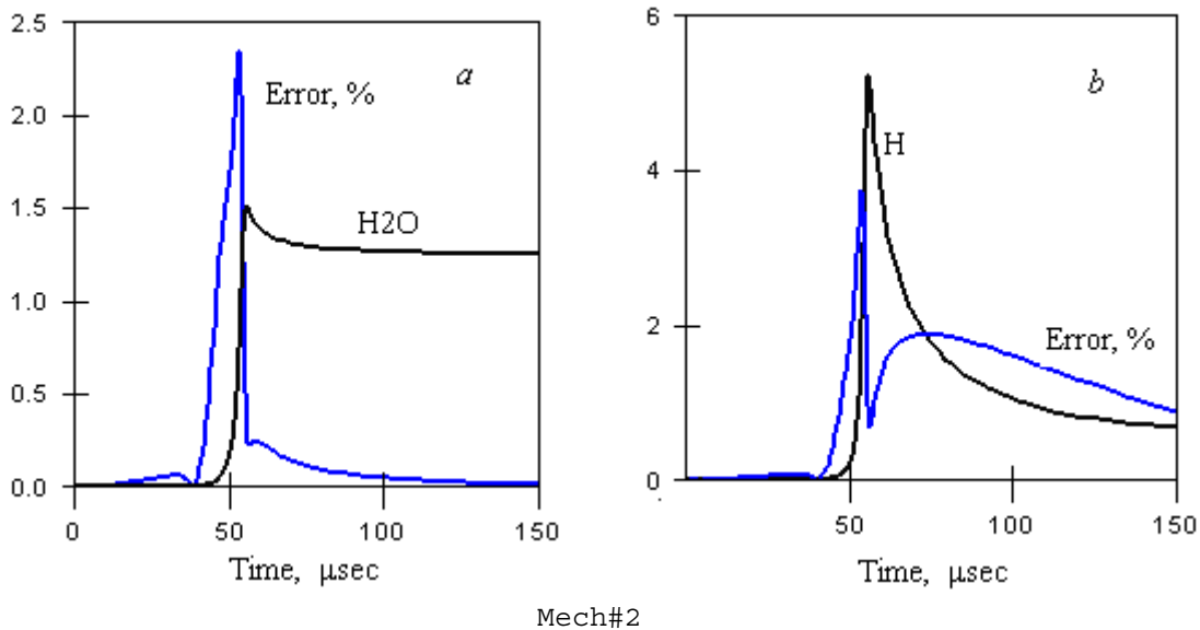
Fig. 2.3. Specie concentration and relative error, %. a – H 2 O concentration, mol/cm 3 × 1.E+6, b – H concentration, mol/cm 3 × 1.E+7.
